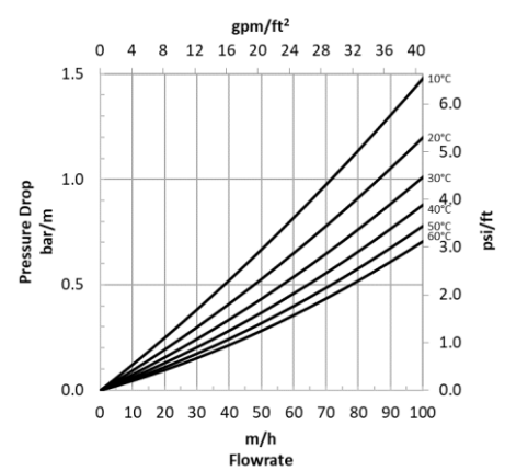
Figure 2: Pressure Drop
