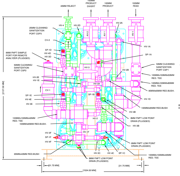
CATHODE END VIEW
