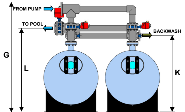
Side by Side (SxS) Dual Tank Design
